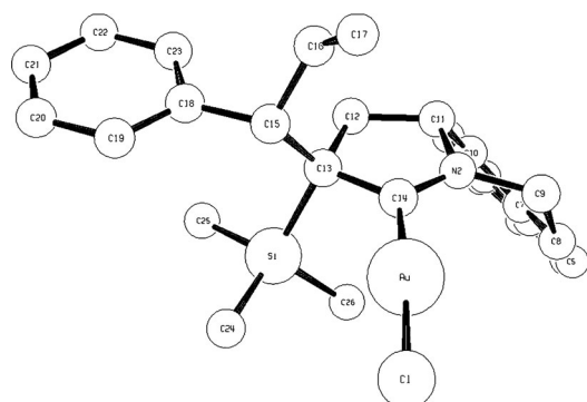
Figure 2. ORTEP of CAAC–Au I complex 2d ; ellipsoids set at 50 % probability. Hydrogen atoms are omitted for clarity. C14–Au–Cl 176.4°, C14–Au 1.985 Å, C14–C13 1.488 Å, C14–N2 1.291 Å, N2–C14–C13 111.2°, C13–Si 1.939 Å.
